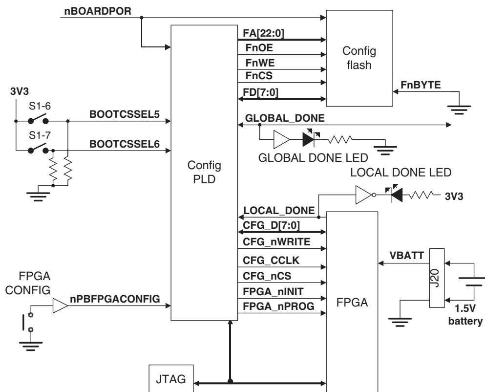
Figure 3-9 FPGA configuration
