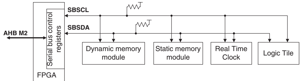
Figure 3-34 Serial bus block diagram
