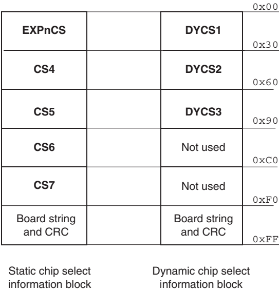
Figure E-4 Chip select information block
