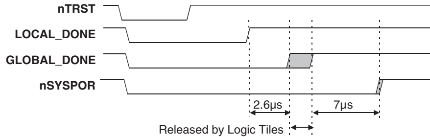
Figure 3-10 FPGA reload sequence
