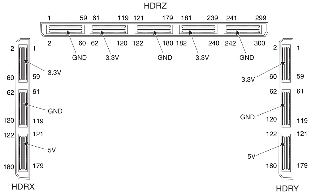
Figure A-14 HDRX, HDRY, and HDRZ (upper) pin numbering
